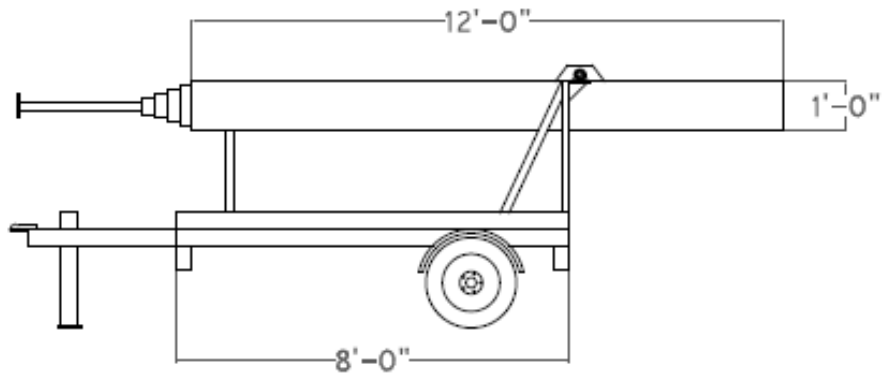
MOBILE MAST
